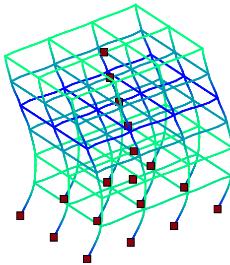
Mode 5 | T = 0.401276 s
