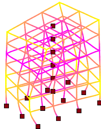
Mode 6 | T = 0.390542 s
