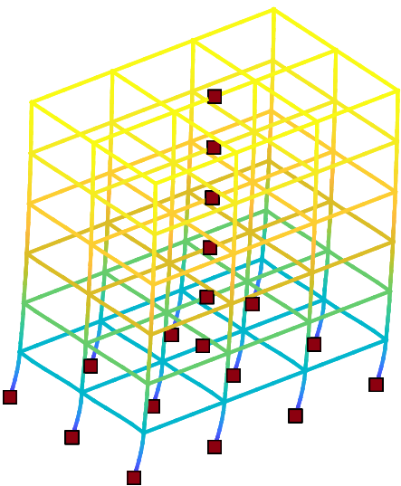
Mode 1 | T = 1.44946 s
