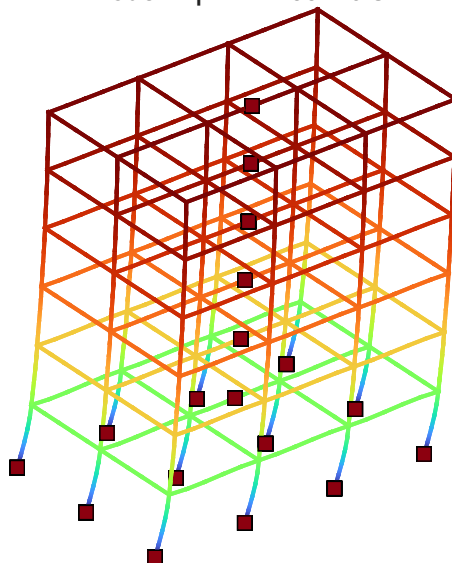
Mode 5 | T = 0.401276 s
