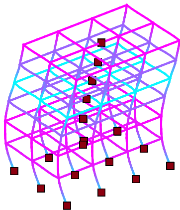
Mode 4 | T = 0.437222 s
