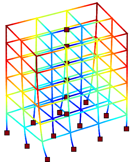
Mode 3 | T = 1.29927 s
